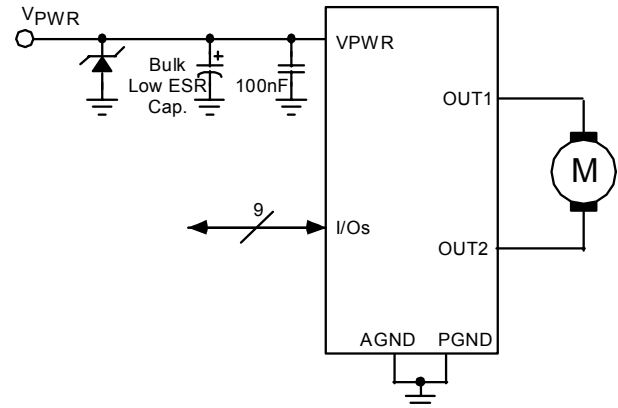
Figure 13. Avalanche Protection
